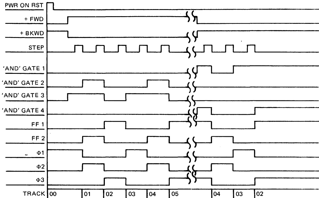
Figure 18 Track Accessing
