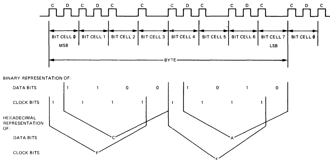
Figure 4 Byte
