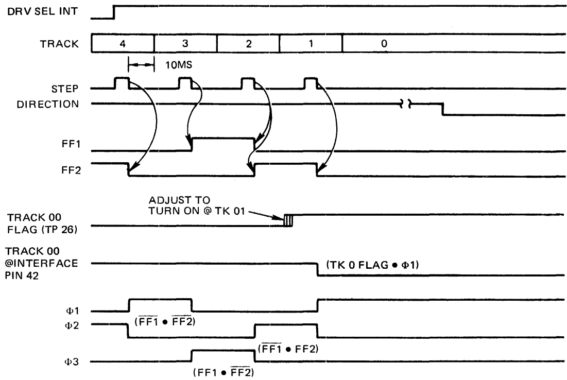
Figure 22 Track 00 Timing
