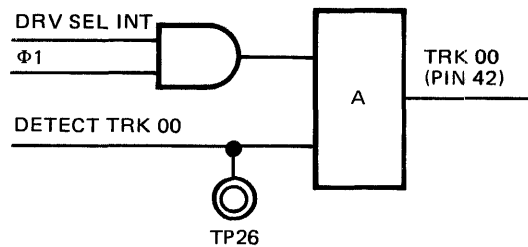
Figure 21 Track 00 Flag
